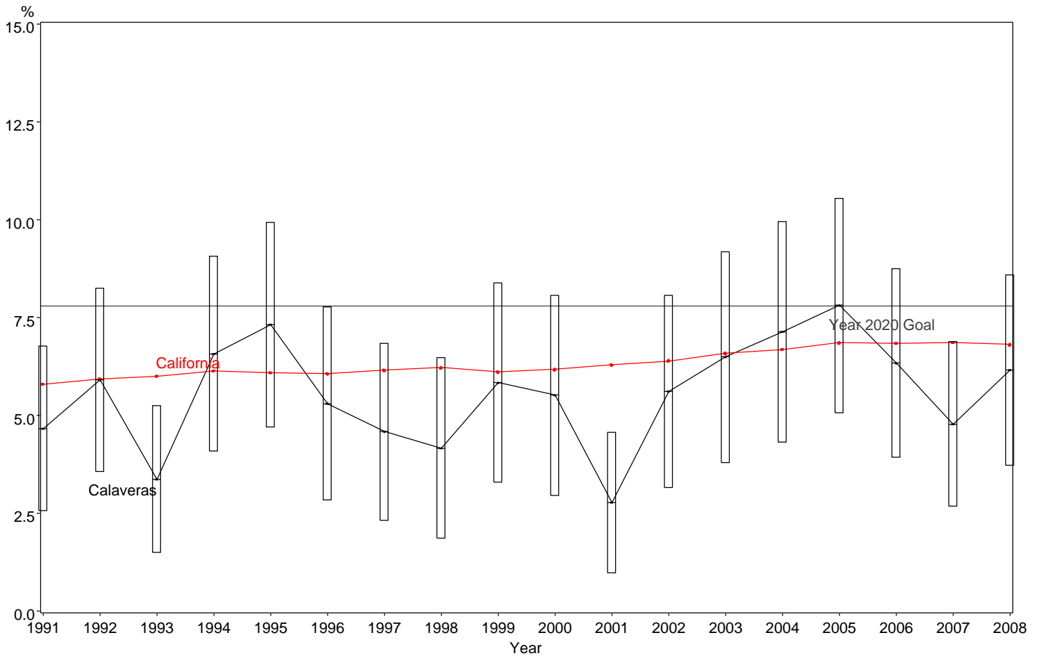
Percent of Low Birth Weight Infants Calaveras County, 1991-2008
