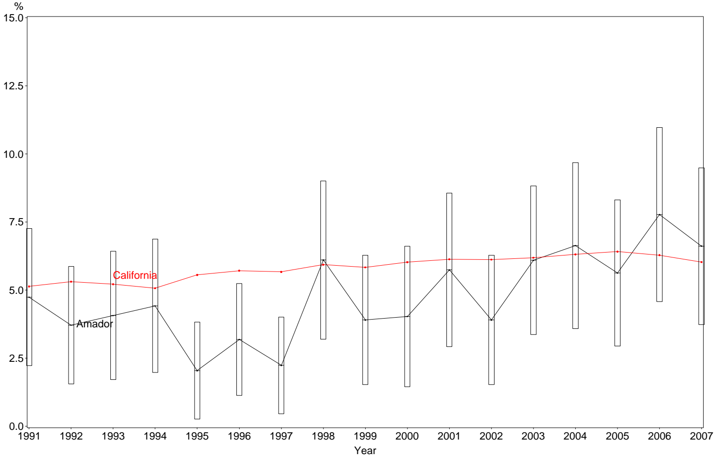
Percent of Newborns with Hospital Stay Longer than 5 Days Until Home Discharge Amador County, 2005-2007
